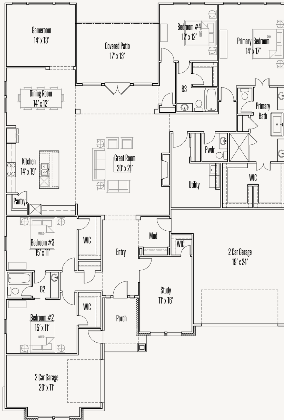
FLOOR PLAN_A
