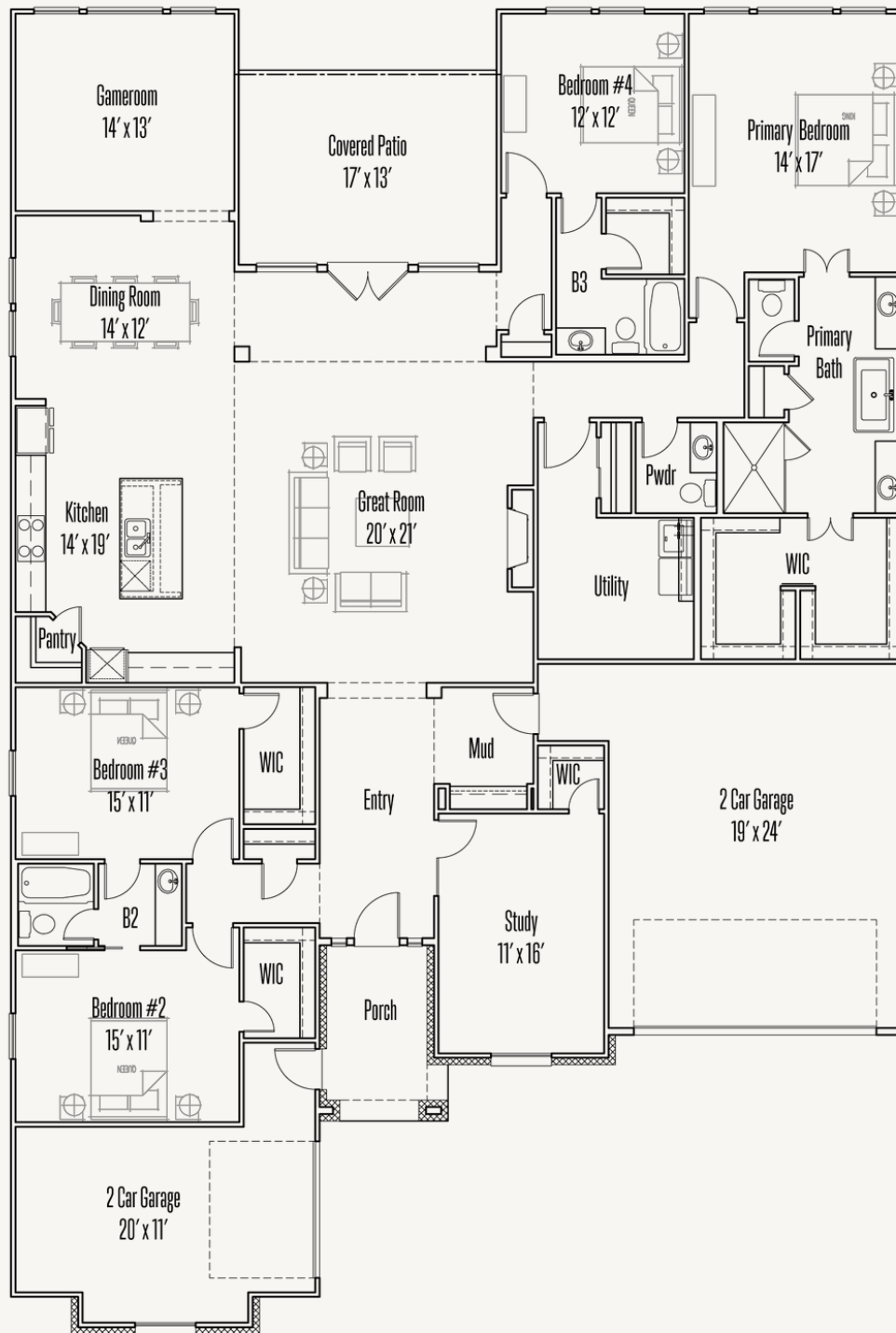
FLOOR PLAN_B
