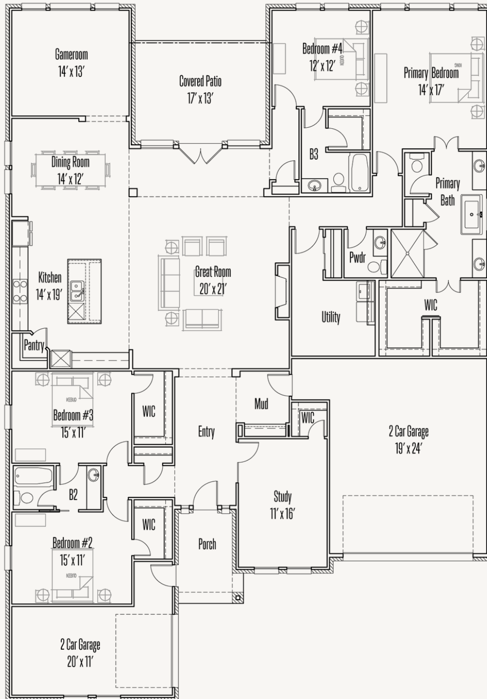
FLOOR PLAN_D
