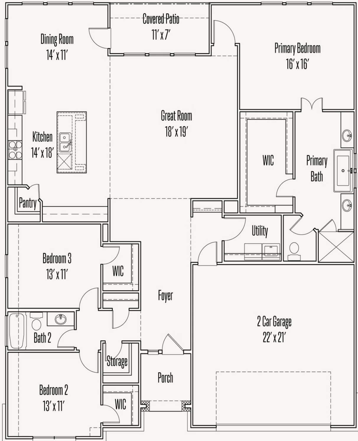
FLOOR PLAN_A
