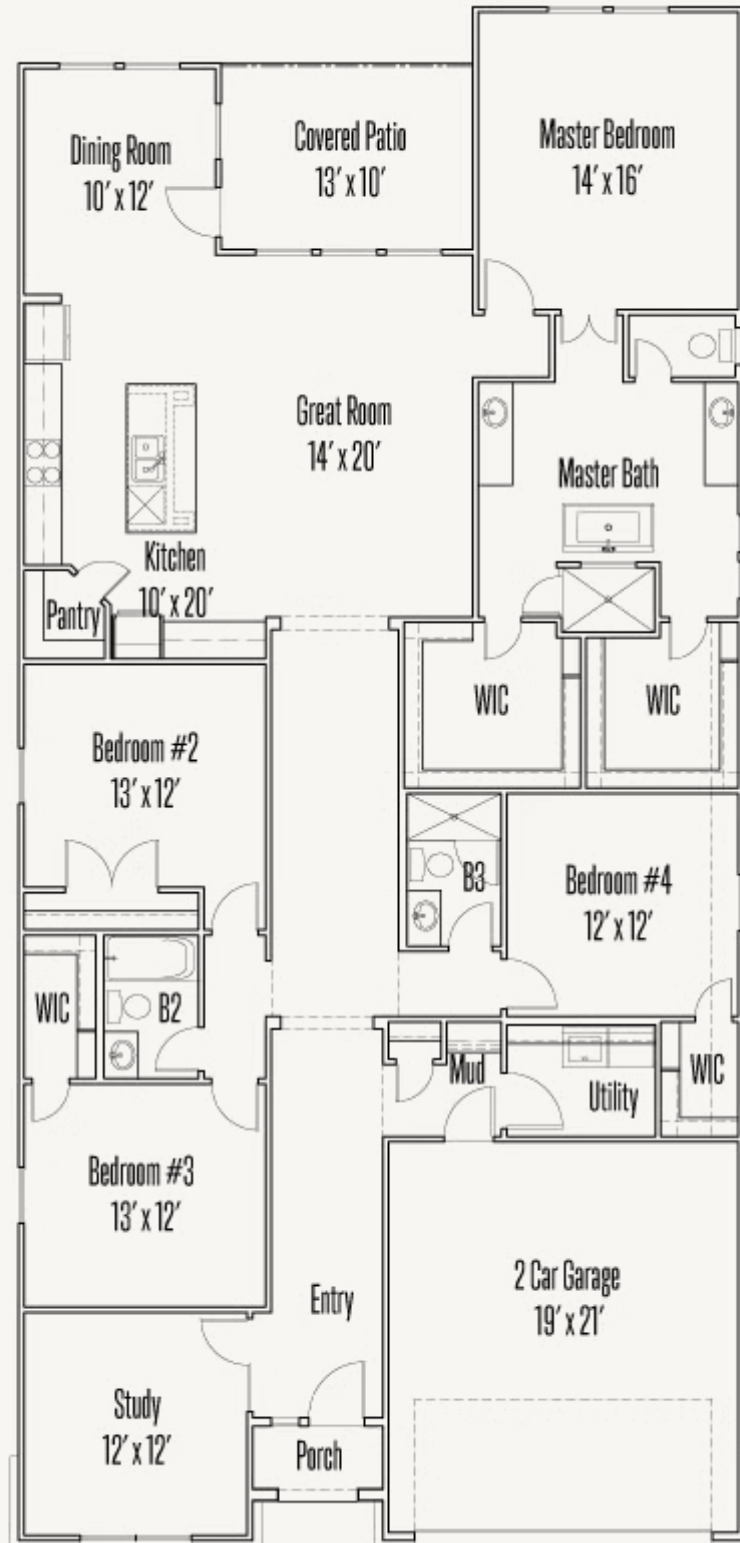
FLOOR PLAN
