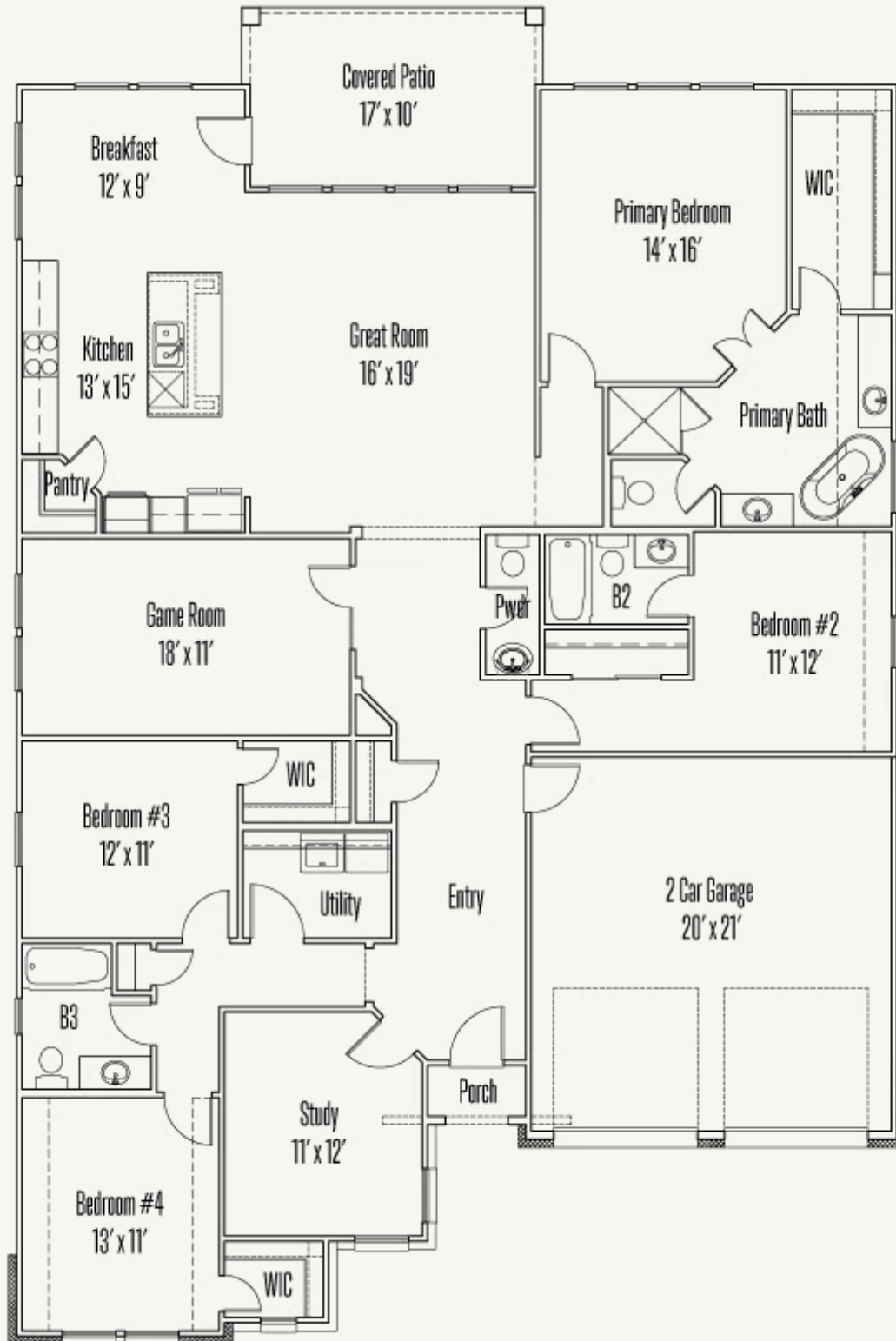
FLOOR PLAN
