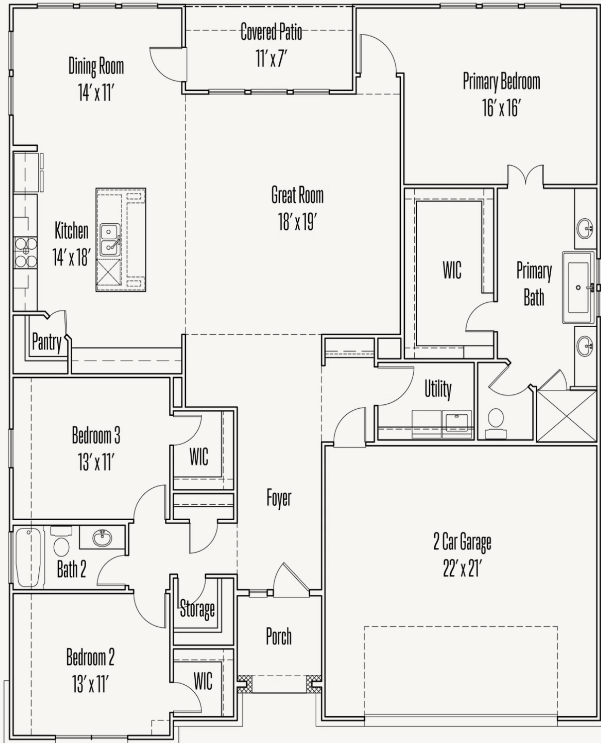
FLOOR PLAN_A
