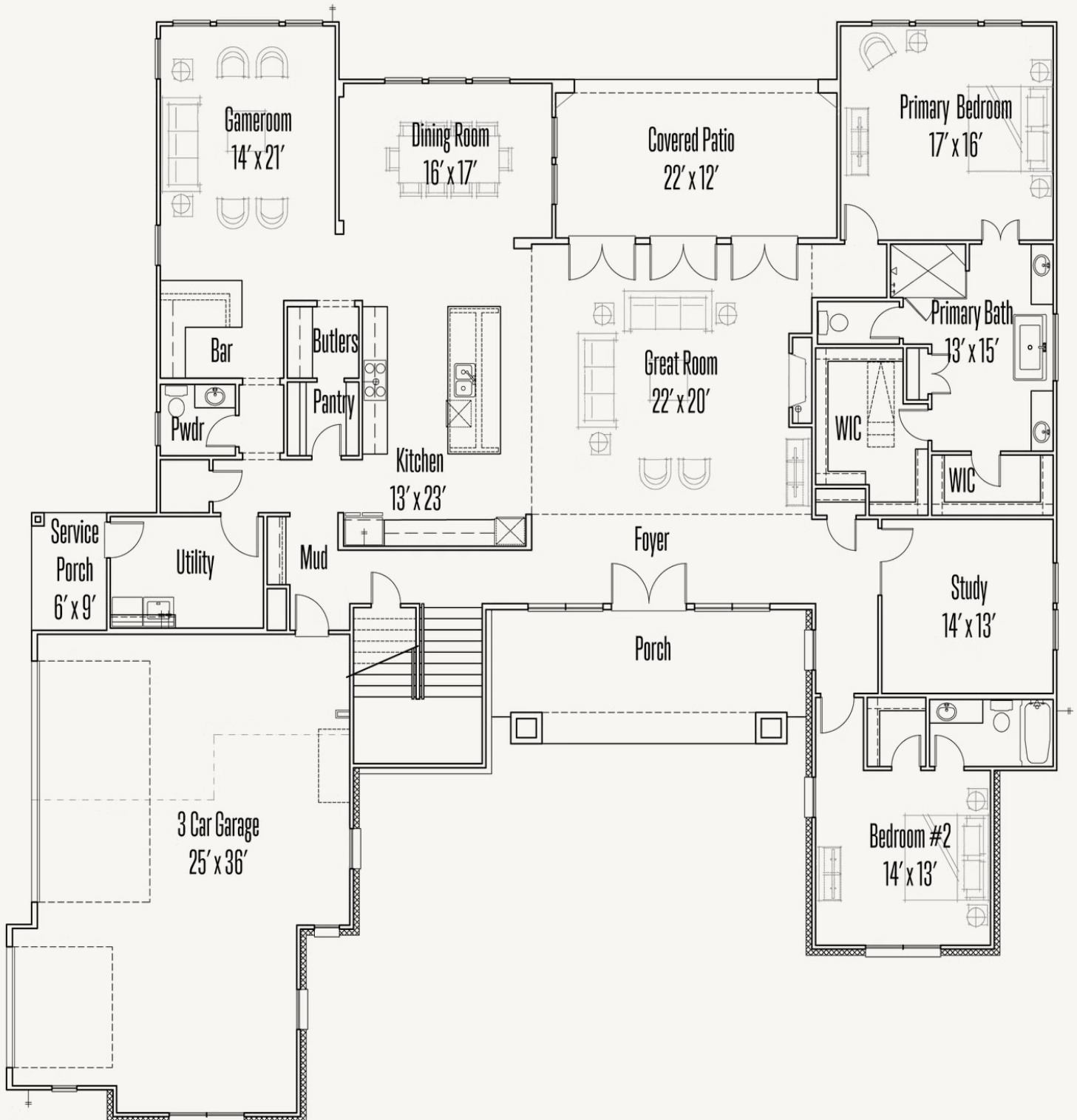
FIRST FLOOR_A
