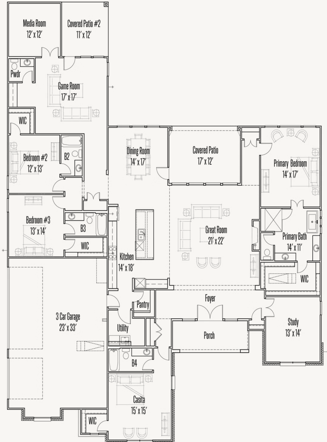
FLOOR PLAN_A
