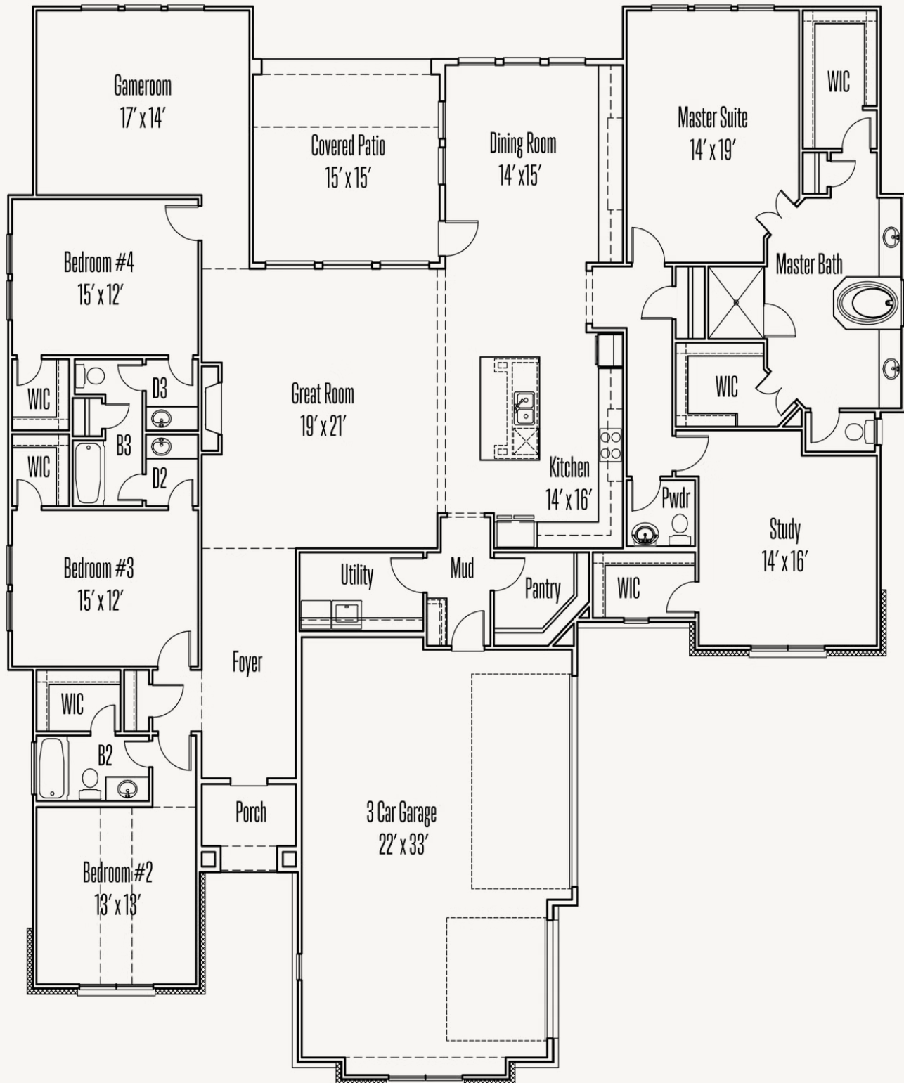
FLOOR PLAN_A
