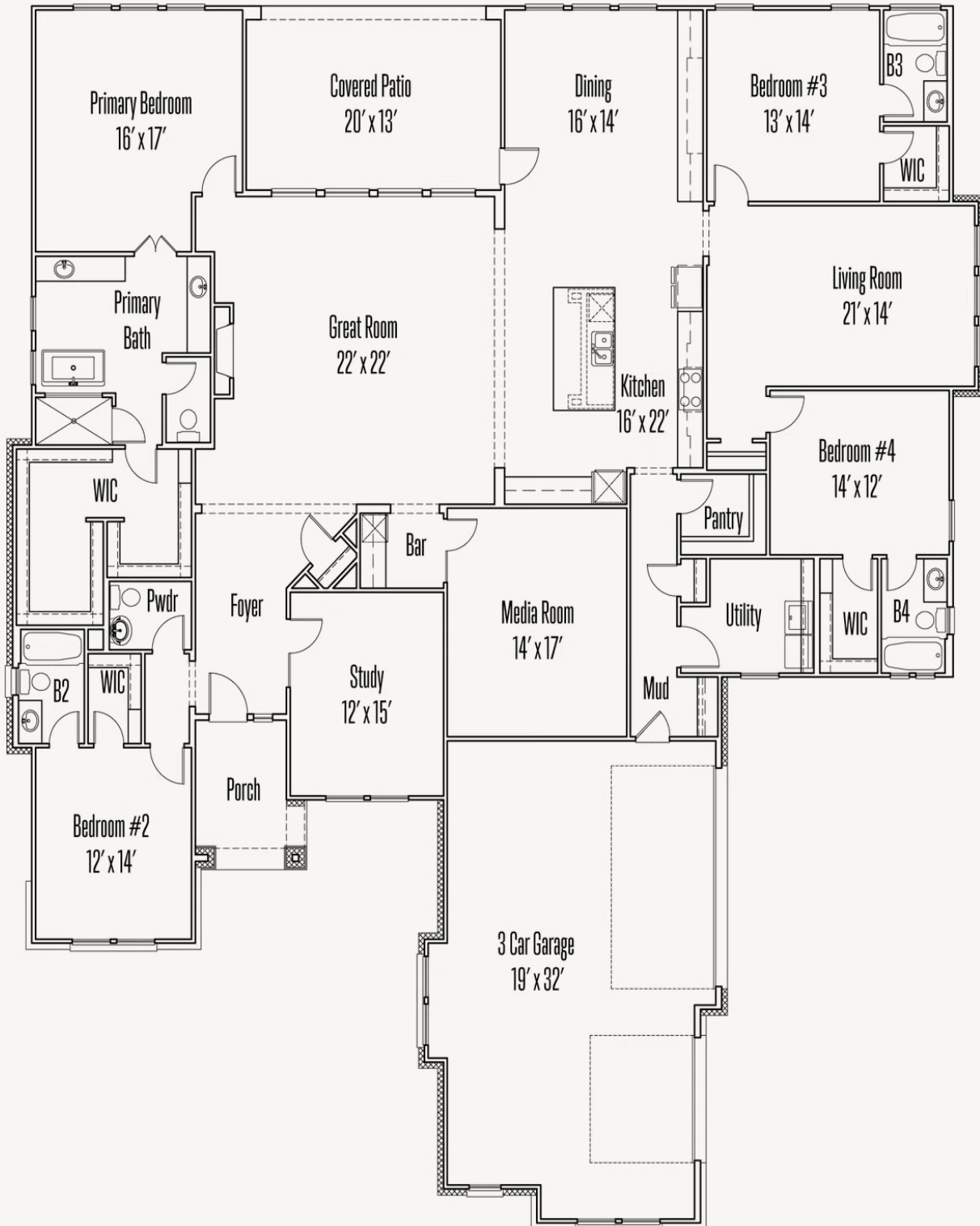
FLOOR PLAN_A
