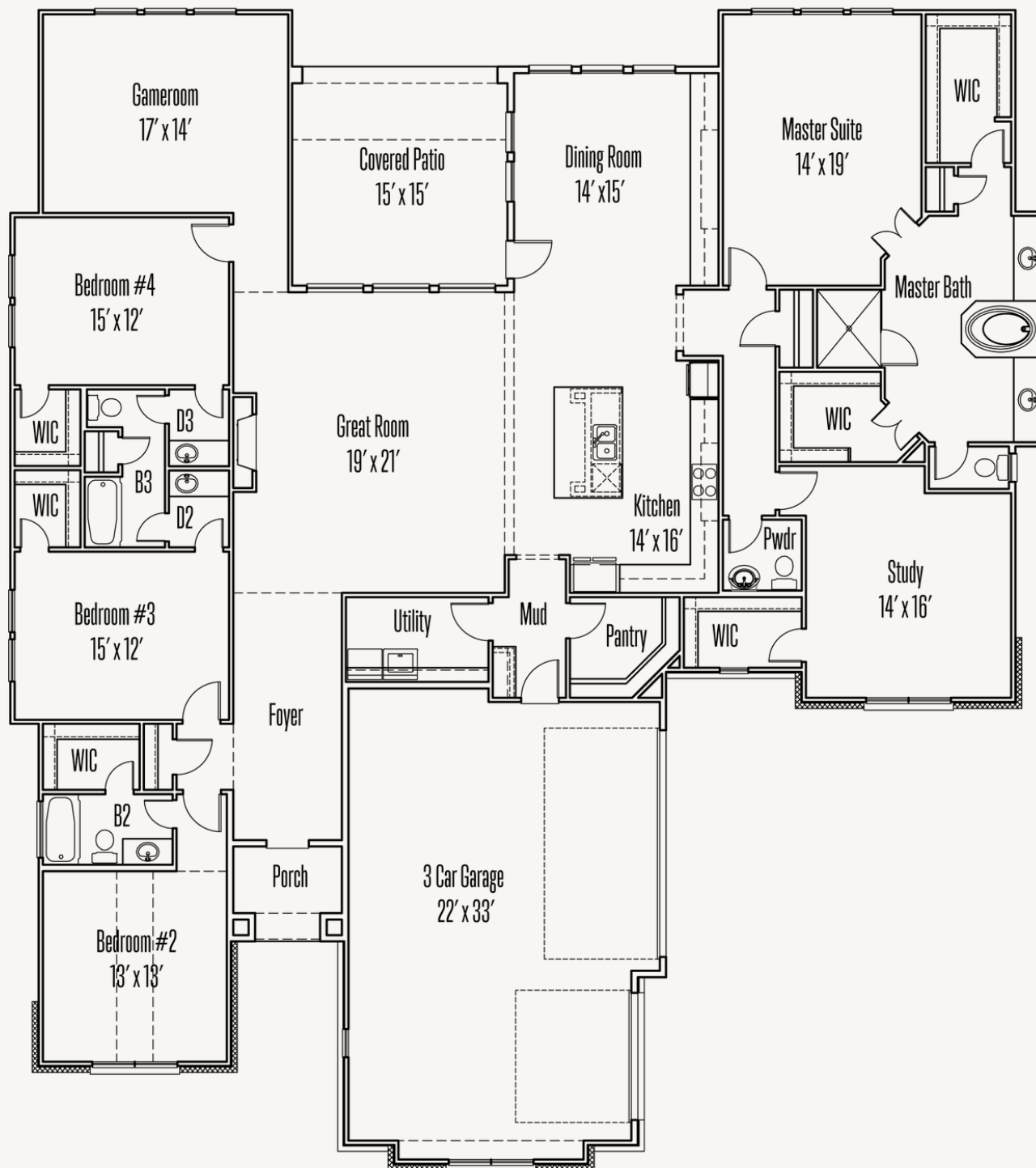
FLOOR PLAN_A
