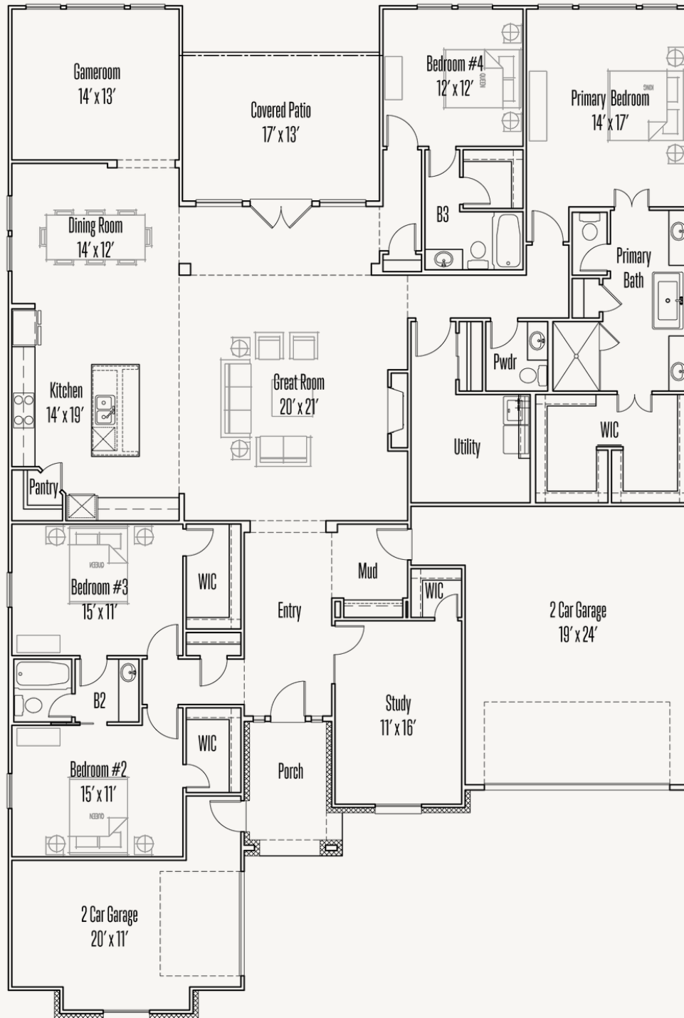
FLOOR PLAN_B
