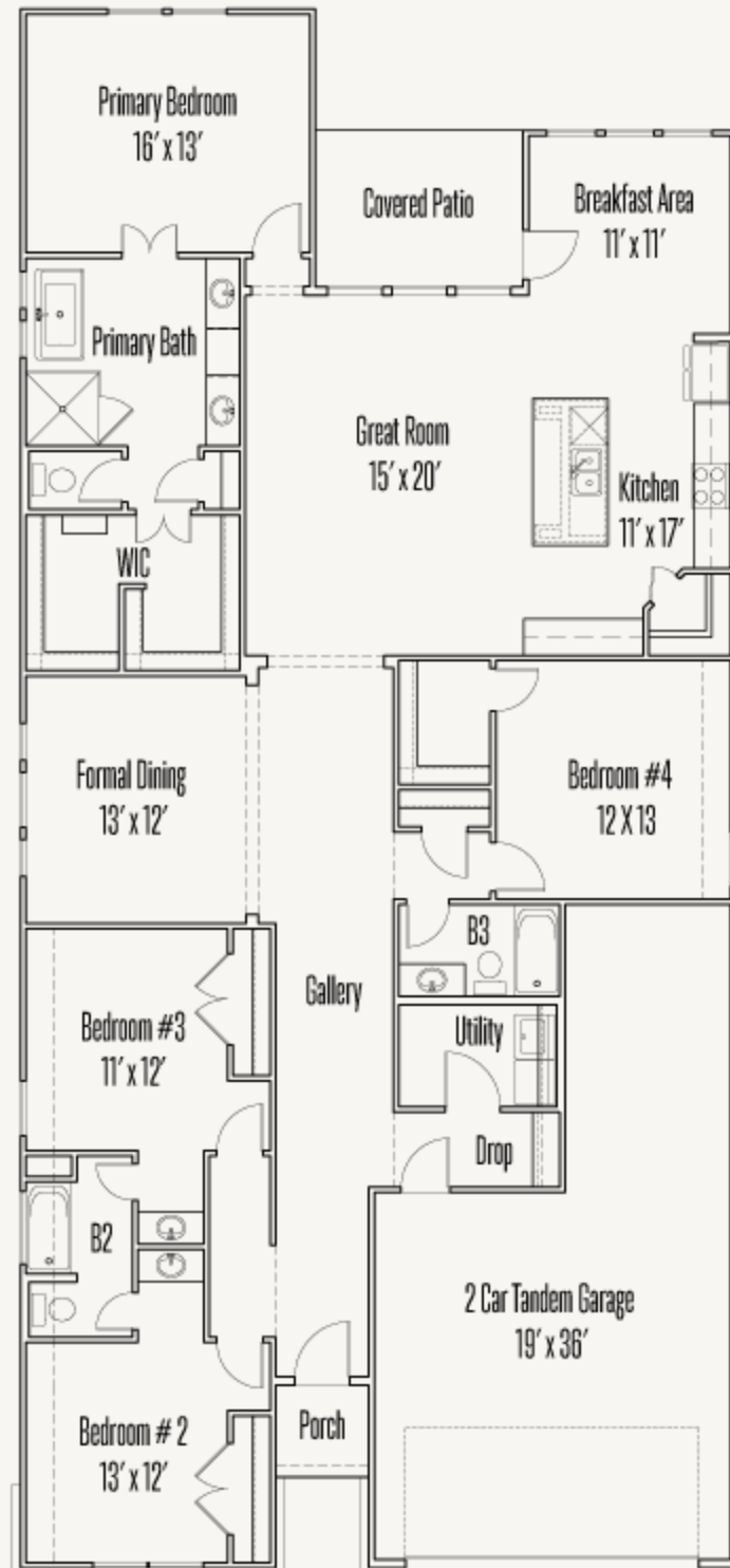
FLOOR PLAN
