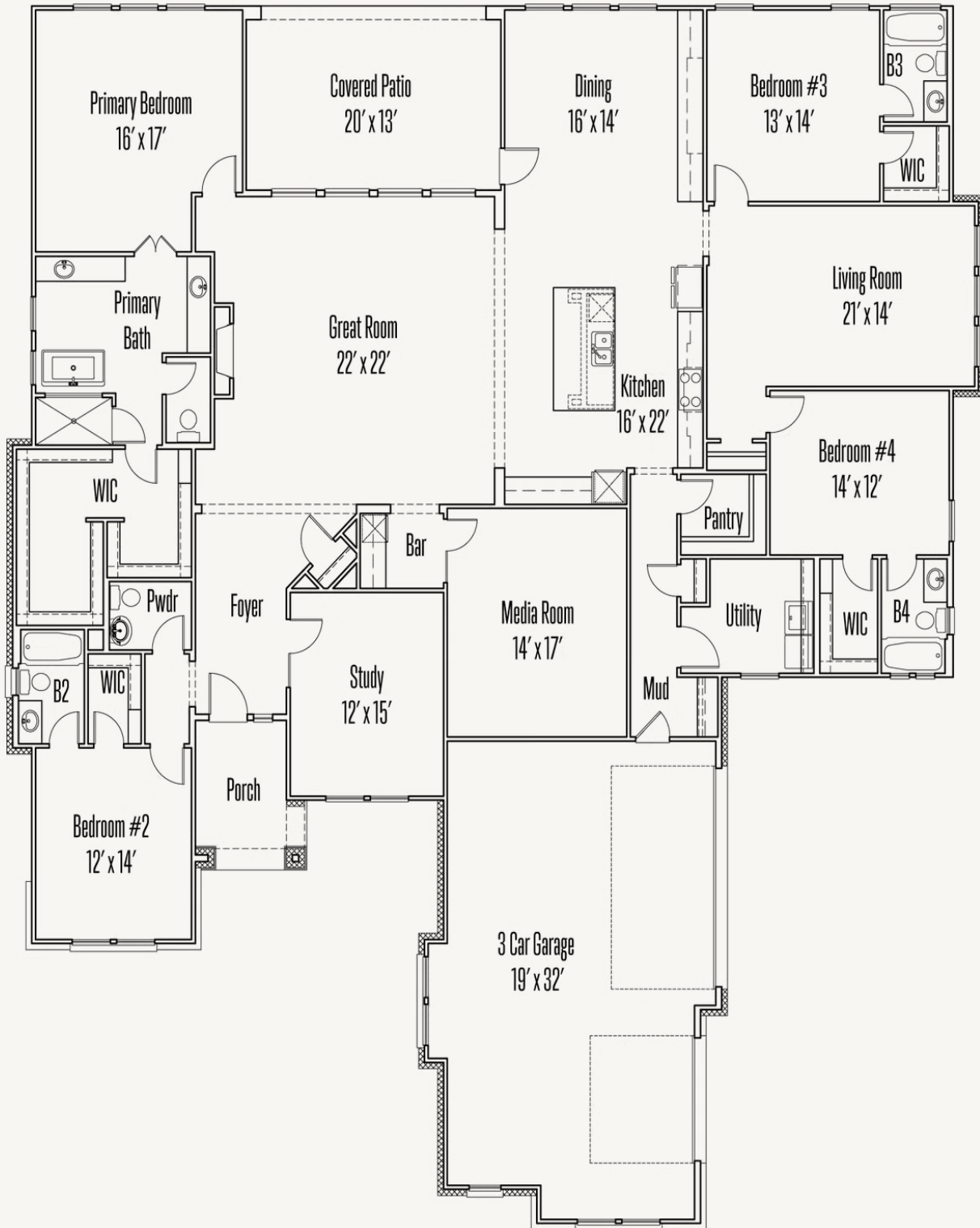
FLOOR PLAN_A
